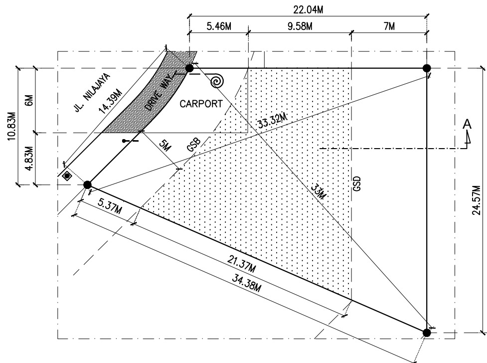
DENAH KAVLING JL. NILAJAYA NO. 19 SKALA 1 : 350
